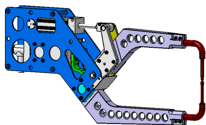
3 Weld guns with aluminum arms
